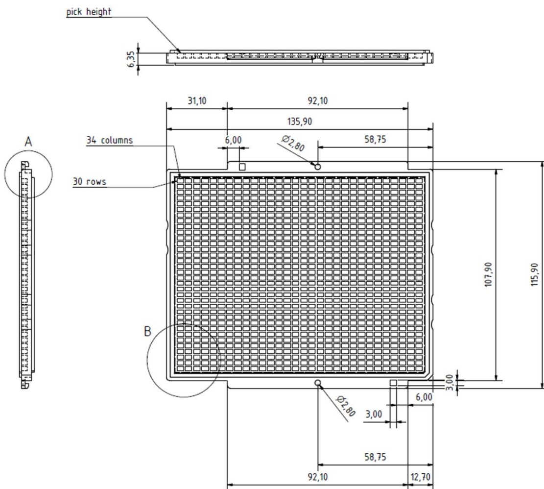
Figure 6: Tray (drawing not to scale)
